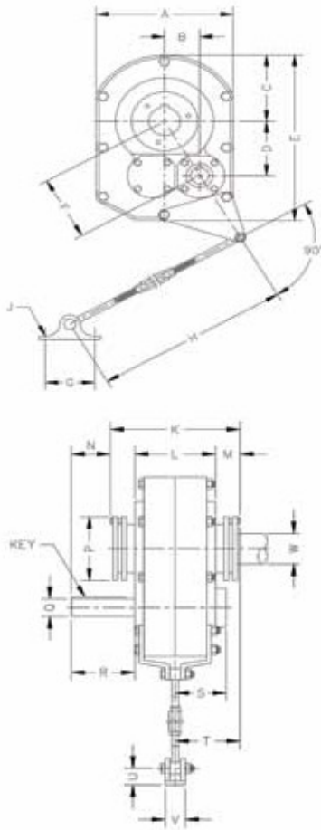
Shaft Mount Reducer
